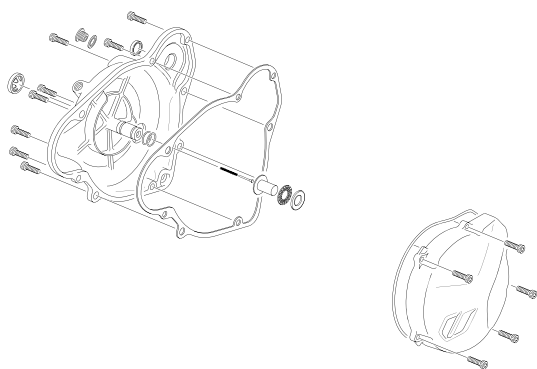
TAPAS - COVERS
