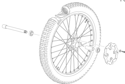
RUEDA DELANTERA - FRONT WHEEL
