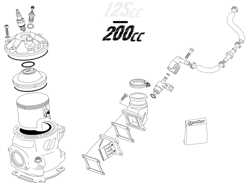
CILINDRO-CULATA-PISTON - CYLINDER-HEAD-PISTON
