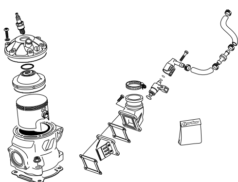
CILINDRO-CULATA-PISTON - CYLINDER-HEAD-PISTON
