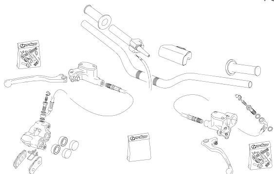
MANILLAR - HANDLEBAR
