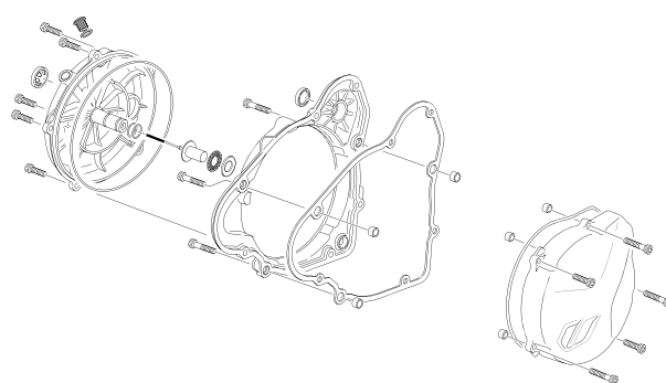
TAPAS - COVERS
