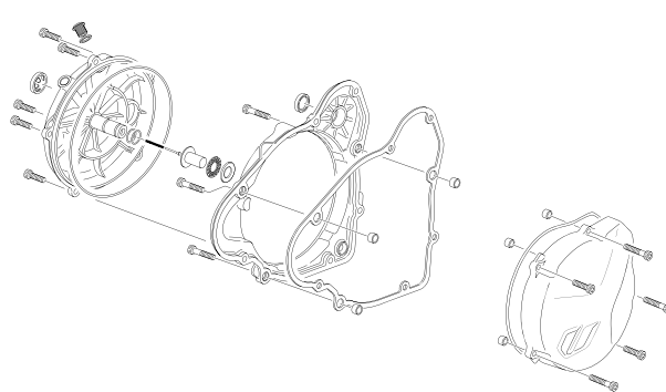
TAPAS - COVERS
