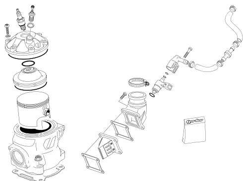
CILINDRO-CULATA-PISTON - CYLINDER-HEAD-PISTON
